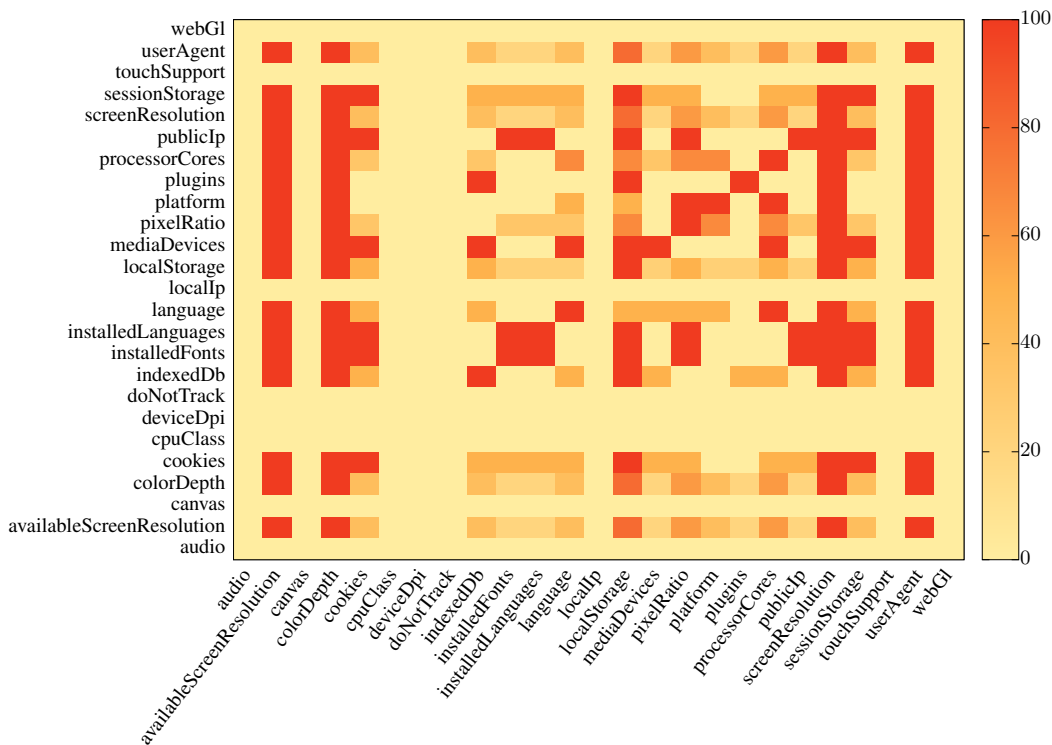
(a) Authentication
